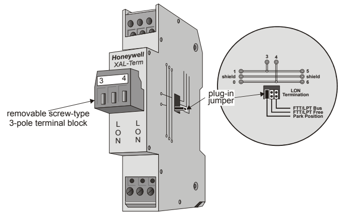
Fig. 13. Lonworks® connection and termination module
