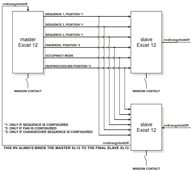
Fig. 5. Master/slave functionality and window contact
