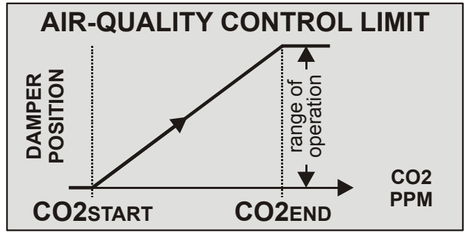
Fig. 3. Air-quality control (example)
