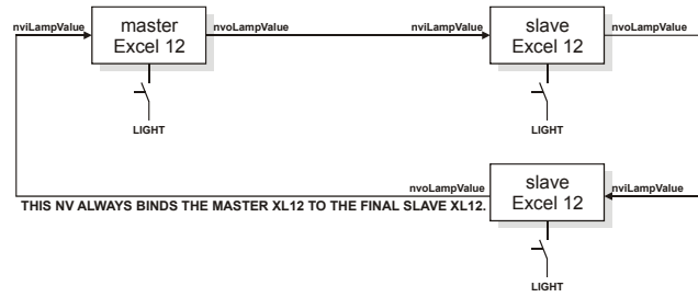
Fig. 7. All lights switched on via any pushbutton
