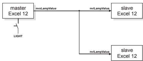
Fig. 6. All lights switched via master pushbutton
