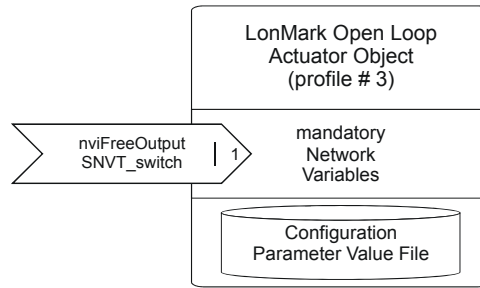
Fig. 9. Open Loop Actuator Object
