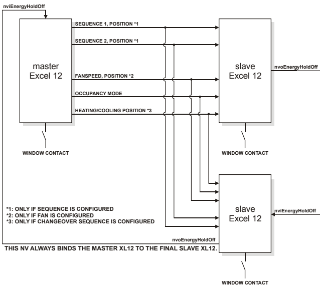
Fig. 2. Master / Slave functionality
