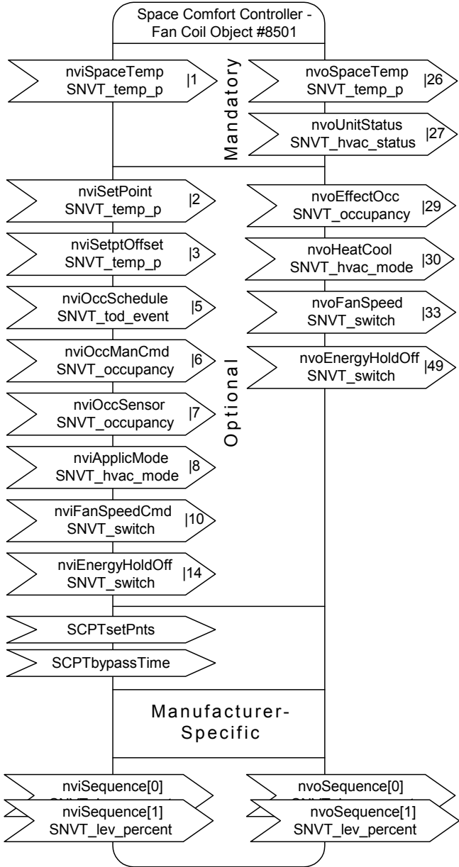
Fig. 11. FCU Controller Object
