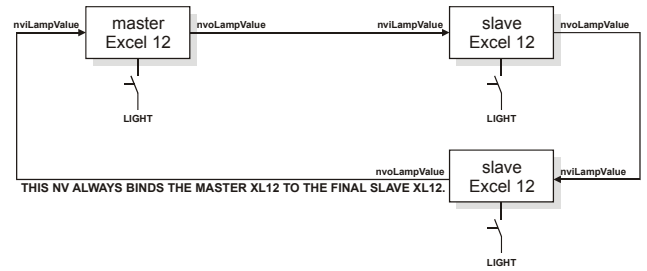
Fig. 4. All lights switched on via any pushbutton
