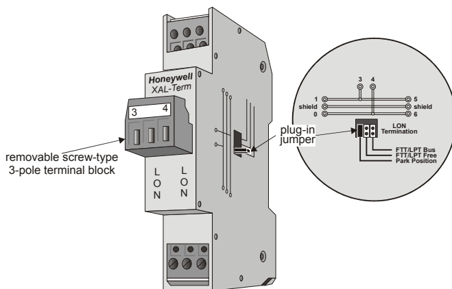
Fig. 13. Lonworks® connection / termination module
