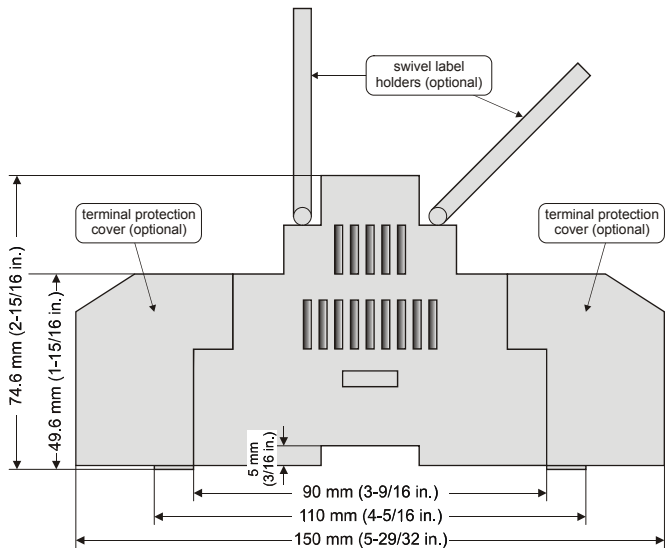
Fig. 1. Excel 12 housing (side view)
