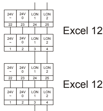
Fig. 9. Connection to LonWorks (fixed terminals)
