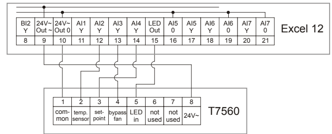
Fig. 7. Wall module connection
