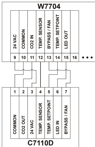
Fig. 8. Connection of C7110D1009
