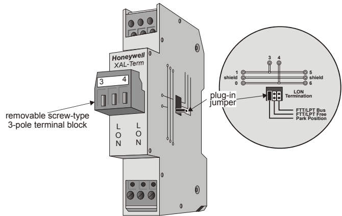
Fig. 11. LONWORKS connection and termination module
