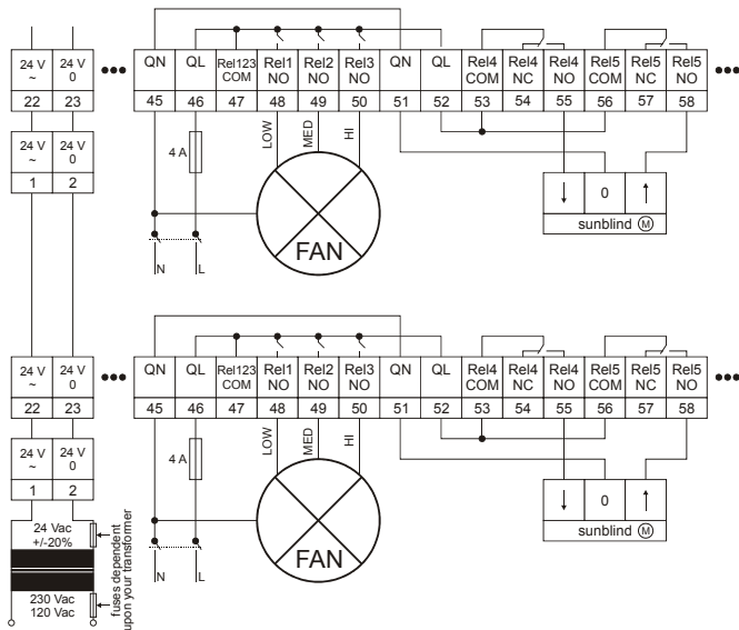
Fig. 6. Connection to 24 Vac power supply
