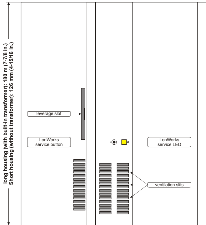
Fig. 10. Housing (top view)
