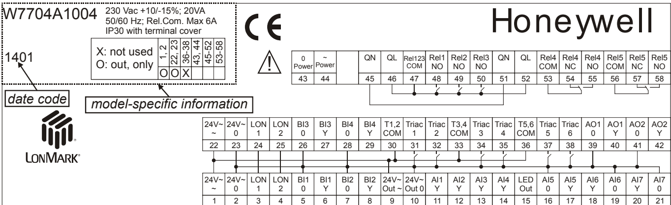
Fig. 4. Example terminal assignment label for W7704A1004
