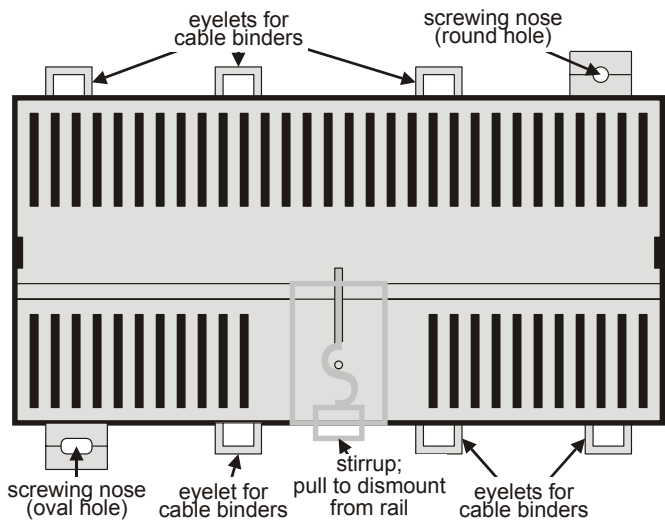
Fig. 2. Housing base (view from below)
