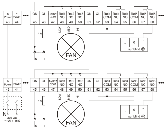
Fig. 5. Connection to 230 Vac power supply
