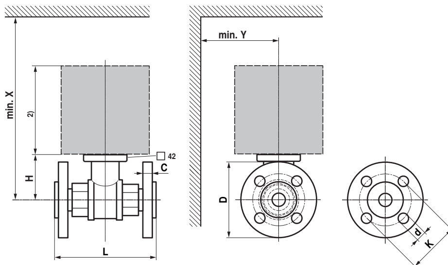
Dimensional drawings
