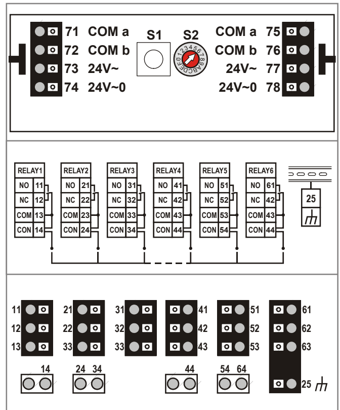
Fig. 18. LION Relay Output Modules (schematic)
