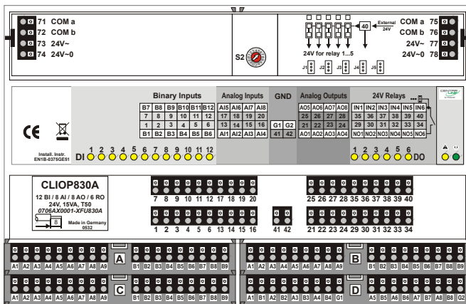
Fig. 22. CLIOP830A mixed Panel Bus I/O module, shown with 4 optional aux. terminal blocks (top view)
