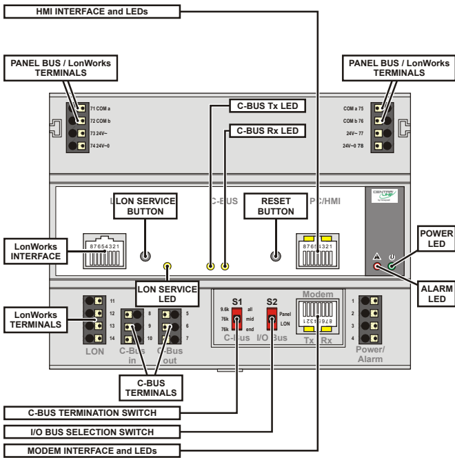
Fig. 4. CLLIONLC01 Controller Module features
