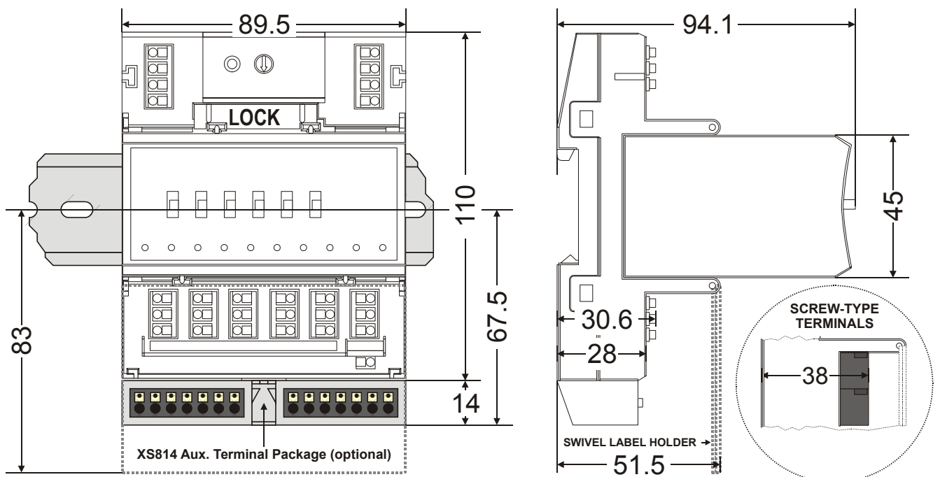
Fig. 24. LION I/O Modules (example shows Manual Overrides), incl. Terminal Socket, outside dimensions (in mm)
