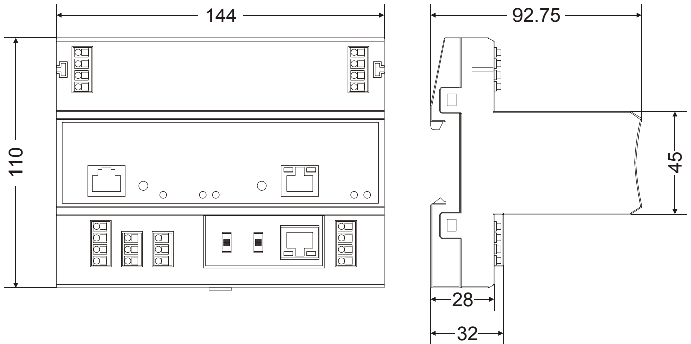
Fig. 23. CLLIONLC01 Controller Module, outside dimensions (in mm)
