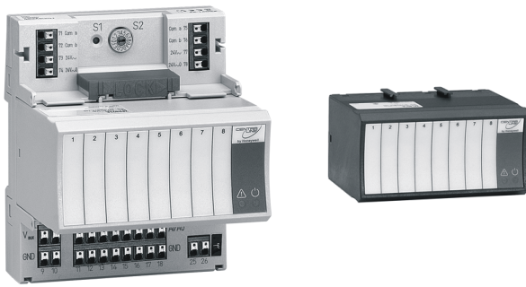
Fig. 9. CLIO821A Panel Bus AI Module (shown with socket) and CLIO821A LonWorks Bus AI Module (shown without socket)
