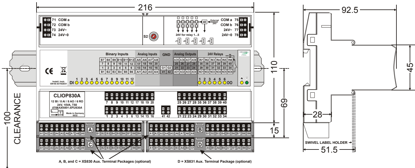
Fig. 25. CLIOP830A mixed Panel Bus I/O module (shown with 4 auxiliary terminal packages), dimensions (in mm)
