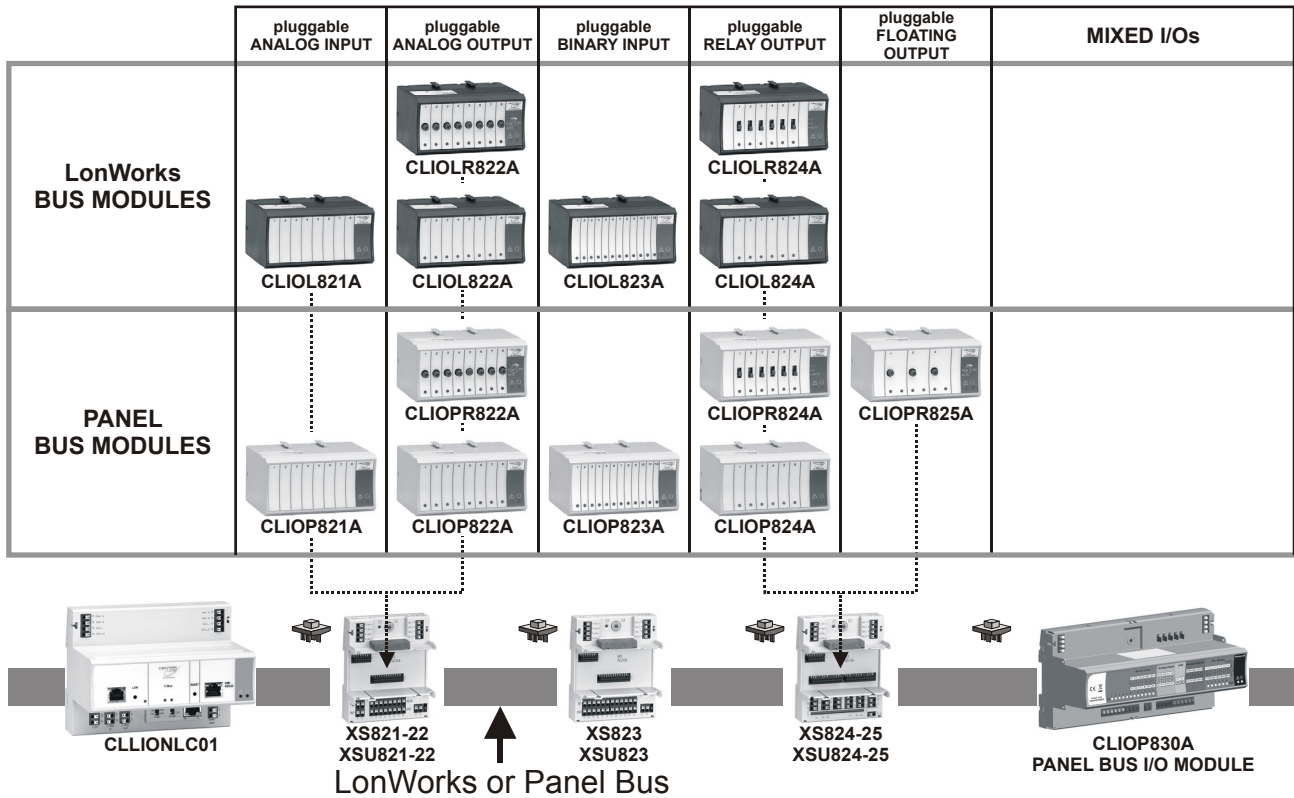
Fig. 2. Overview of LION Modules
