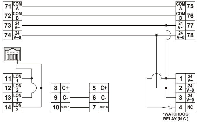
Fig. 5. CLLIONLC01, terminal assignment
