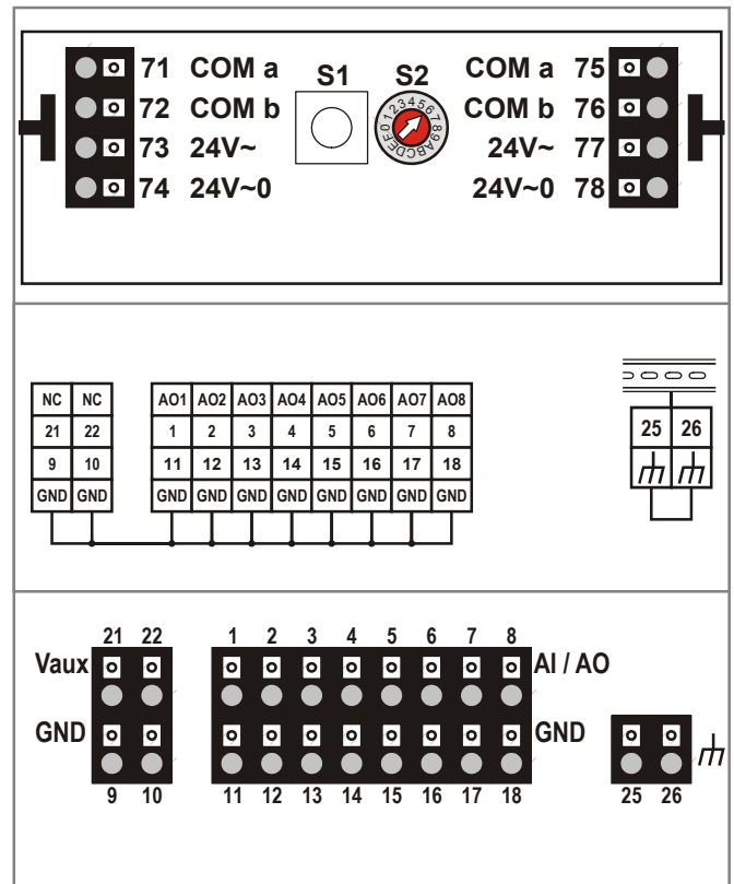
Fig. 13. LION Analog Output Modules (schematic)
