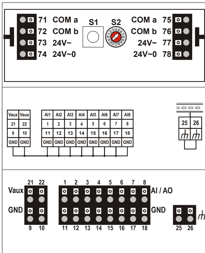
Fig. 10. LION Analog Input Modules (schematic)
