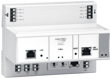
Fig. 3. CLLIONLC01 Controller Module
