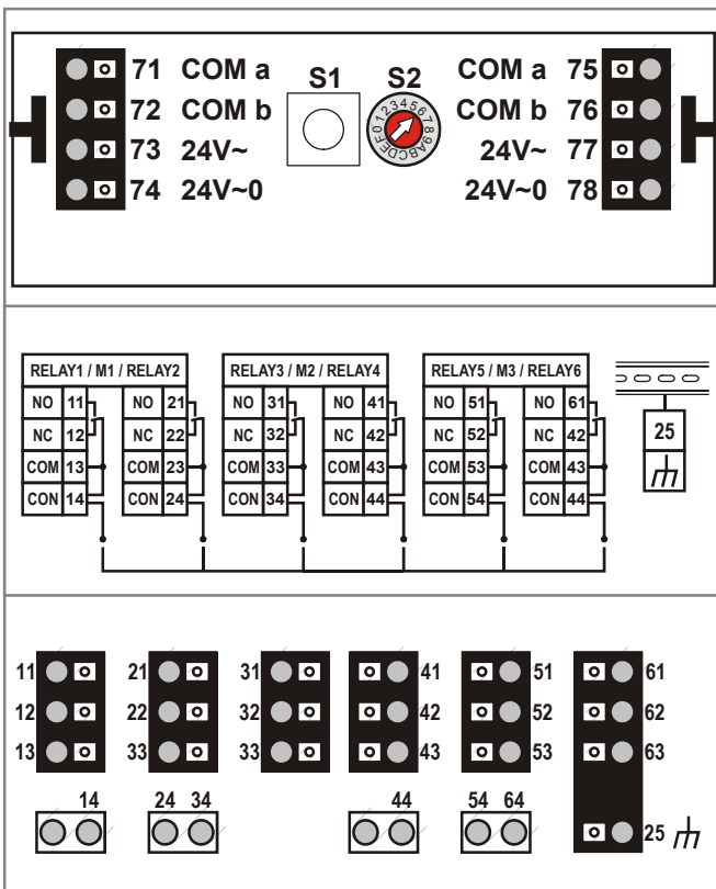
Fig. 20. CLIOPR825A Panel Bus Floating Output Module (schematic)
