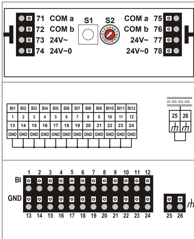
Fig. 15. LION Binary Input Modules (schematic)
