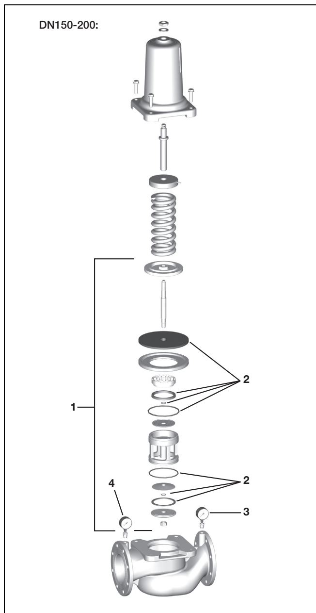
Figure 5: Spare parts
