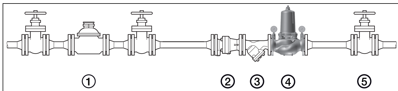
Figure 1: Installation example
