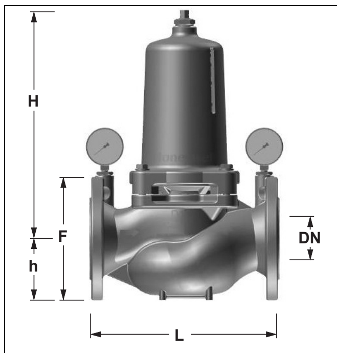
Figure 2: Dimensions
