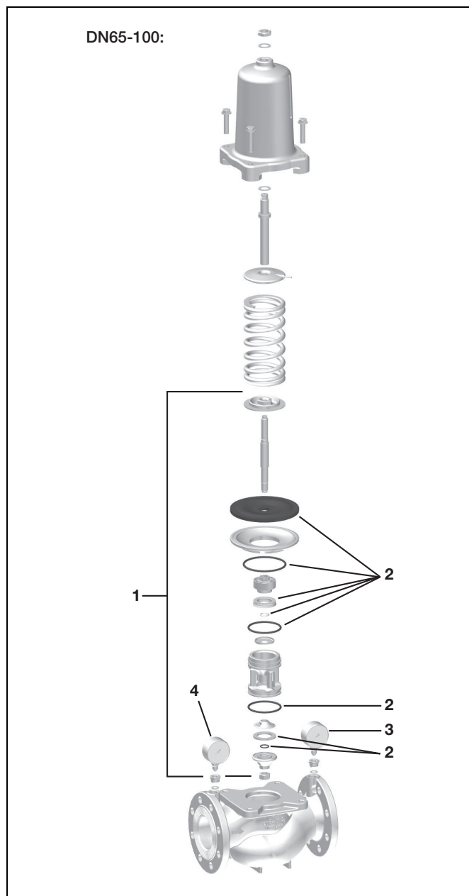
Figure 4: Spare parts
