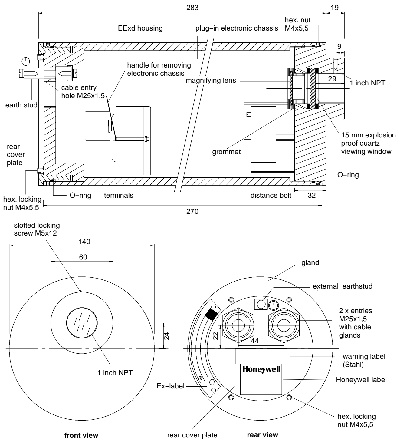
Fig. 6. Dimensional drawing C7076F
